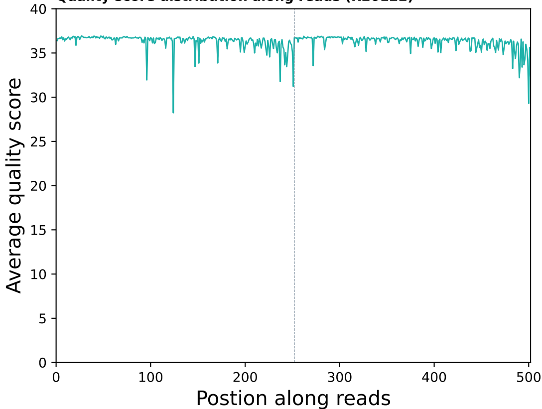
Quality score distribution along reads (R20122)
